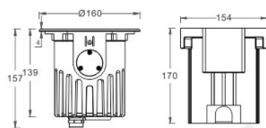
Physical Dimension(MM)
