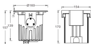
Physical Dimension(MM)
