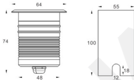
Physical Dimension(MM)
